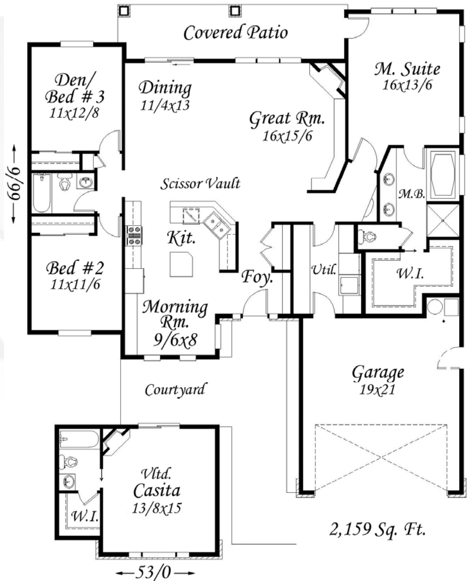
Plan M-2159JTR 53/0p wide x 66/6 deep 2159 sq. ft.
