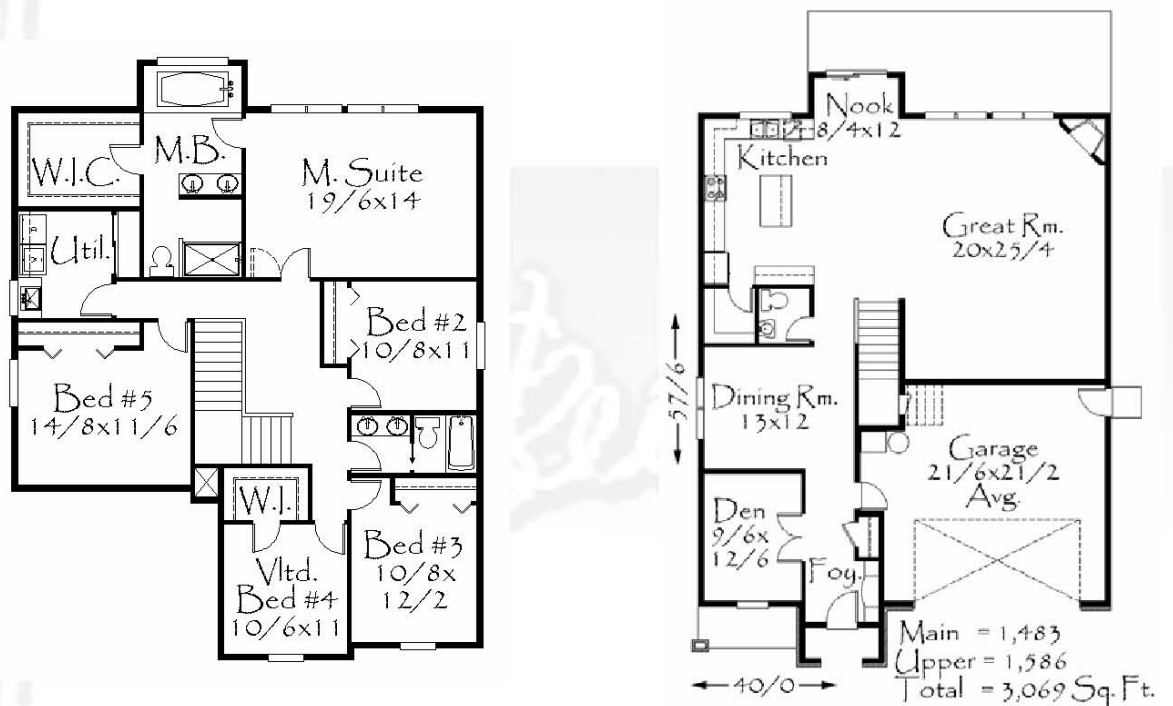
Plan M-3069 40/0 x 57/6 3069 sq. ft. total
