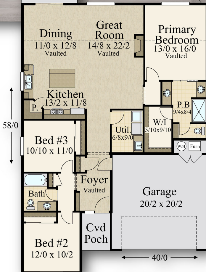
First Floor - 1.703 Sq. Ft
